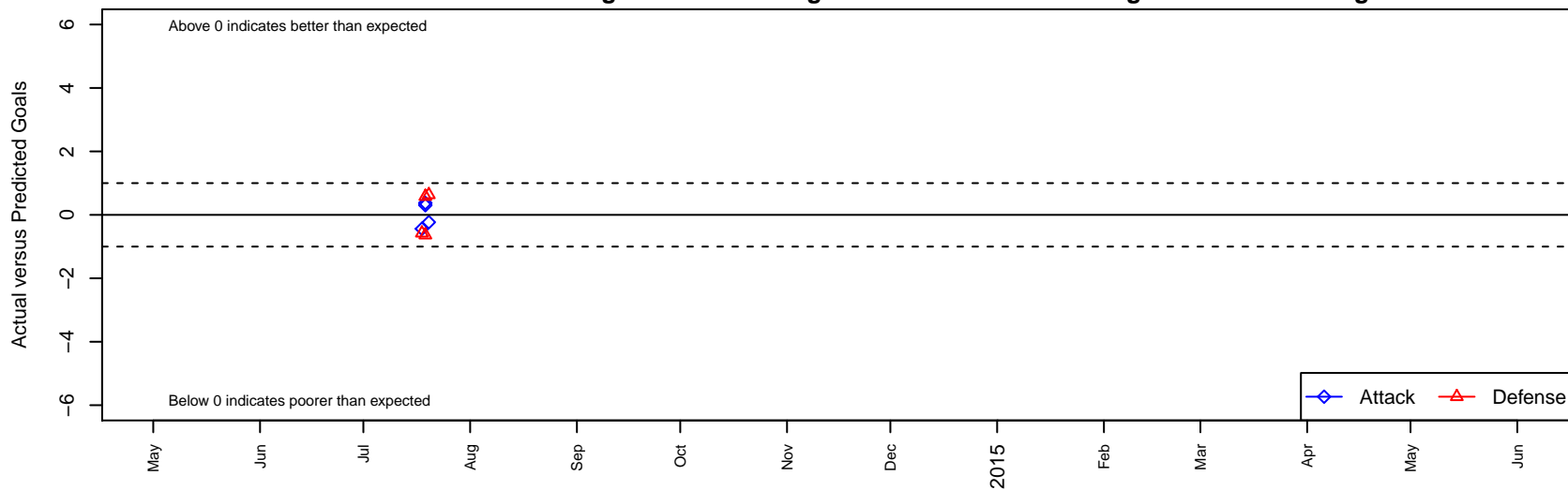
Cook Inlet Velocity 03 White G02 Dots are actual minus expected GF (blue circles) and GA (red triangles). Blue line is smoothed change in attack strength. Red is smoothed change in defense strength.
